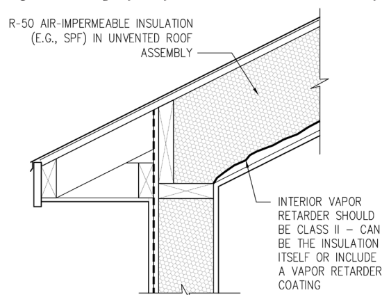
Figure 2.27: Spray Polyurethane Foam (SPF) Cavity Insulation.*
