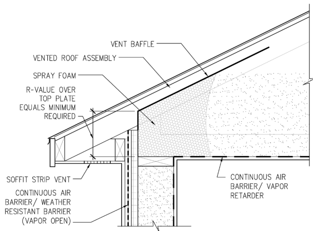
Figure 2.26: Spray Foam above Wall Plate.
