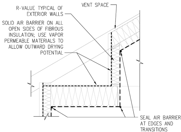
Figure 2.18: Knee Wall Condition, Outside the Building Enclosure.
