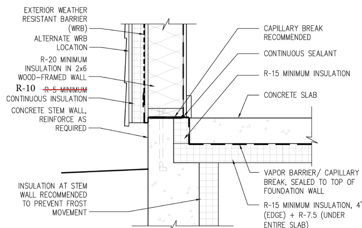
Figure 2.13: Slab Edge Insulation with 2x6 Above-Grade Wall (R-20 + 10 ci Shown).
