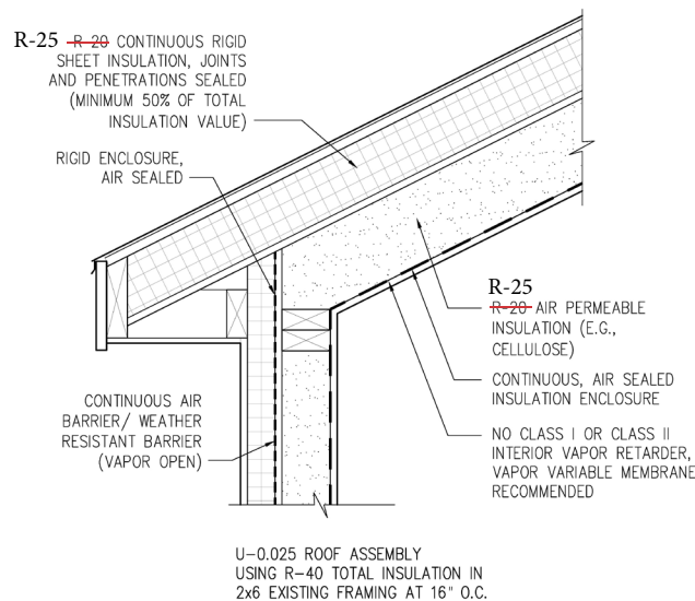
Figure 2.29: Exterior Rigid Board.
