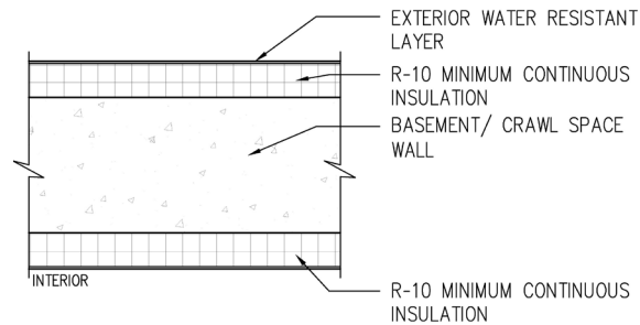
Figure 2.12: Foundation Wall with Interior and Exterior Foam Insulation (Insulated Concrete Form, or ICF).
