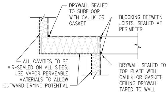
Figure 2.20: Overhanging (Cantilevered) Floor.
