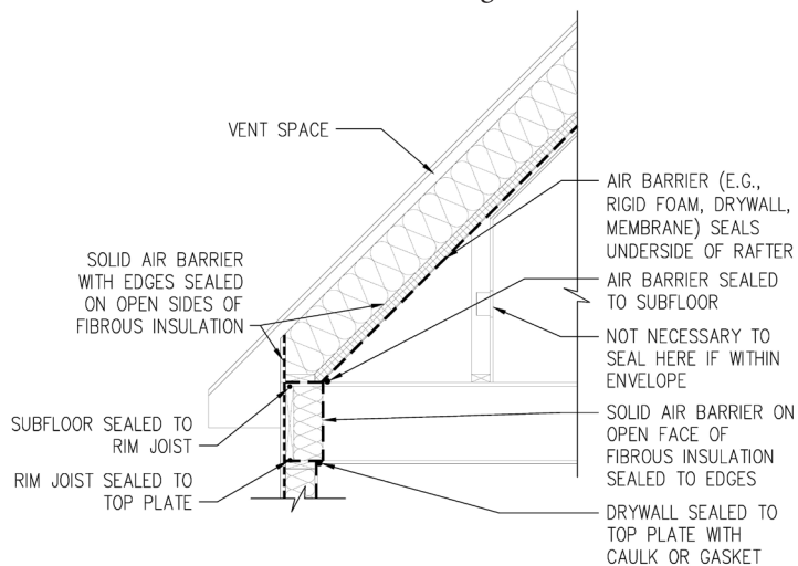
Figure 2.19: Knee Wall Conditions, Inside the Building Enclosure.
