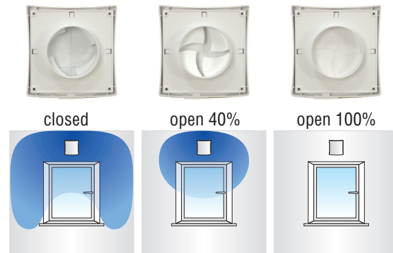
Air flow distribution of depending on different position of the air flow control
