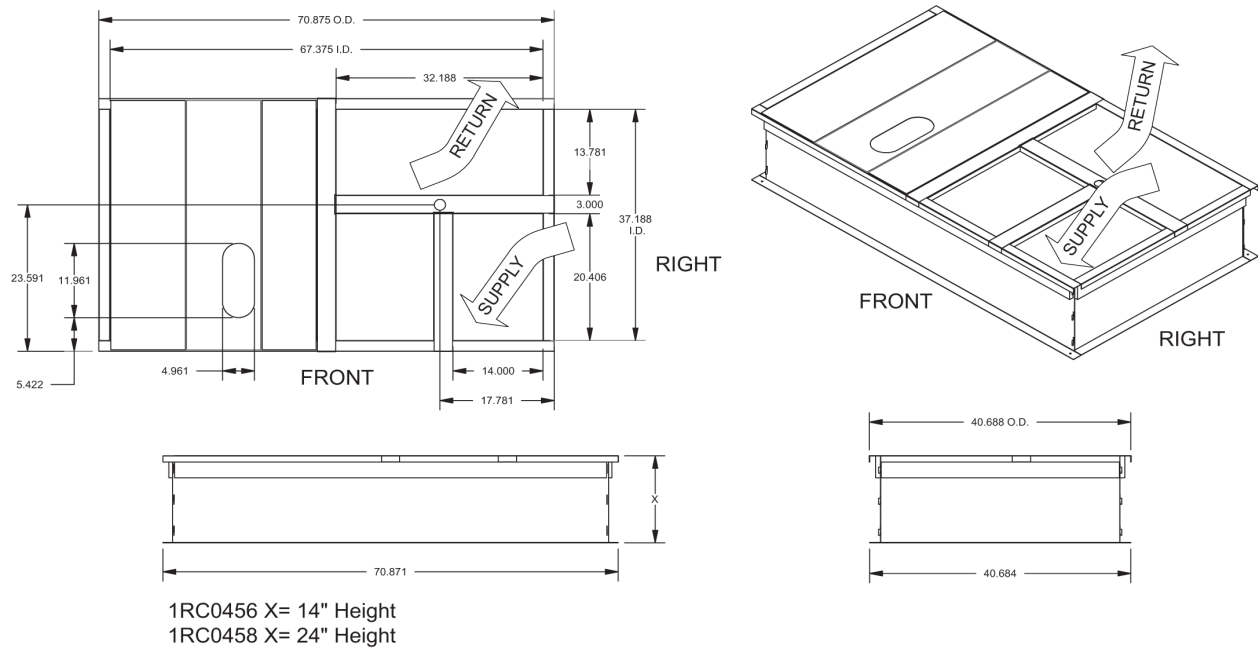
Figure 29: 1RC0456, 1RC0458 roof curb dimensions
