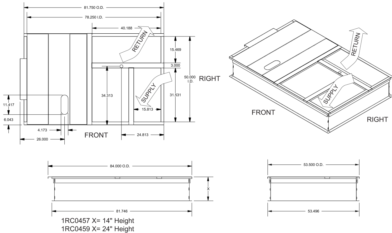
Figure 30: 1RC0457, 1RC0459 roof curb dimensions
