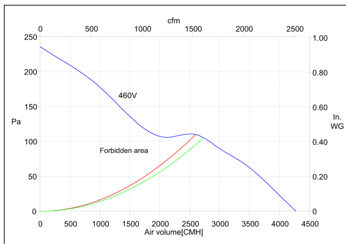
Figure 3: 460-3-60 power exhaust fan curve
