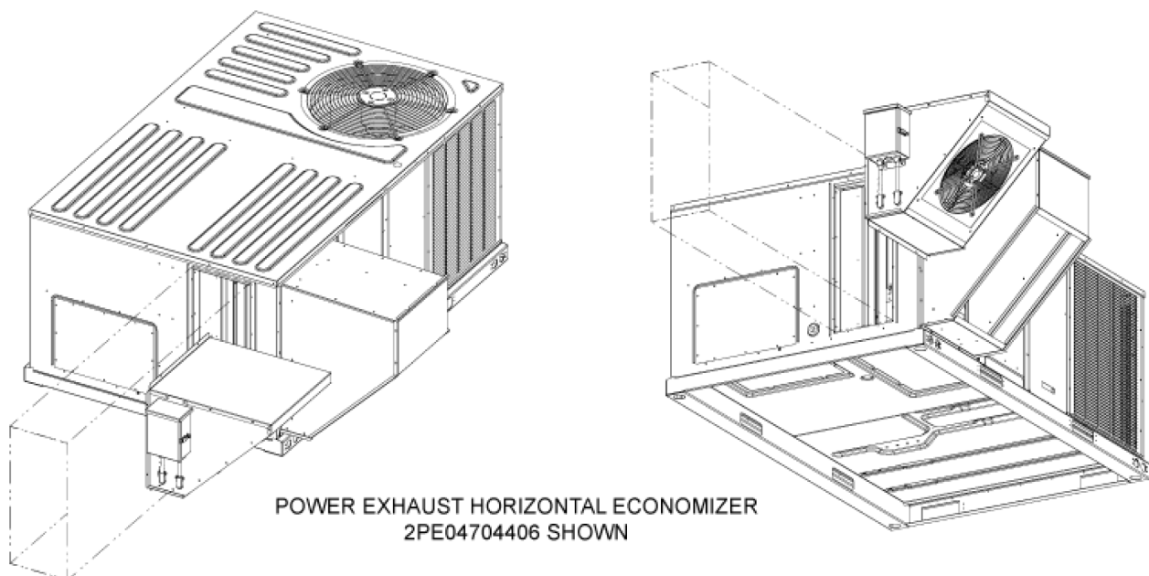
Figure 34: Field-installed horizontal flow economizer w/power exhaust
