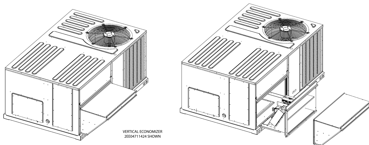
Figure 31: Field-installed vertical flow economizer
