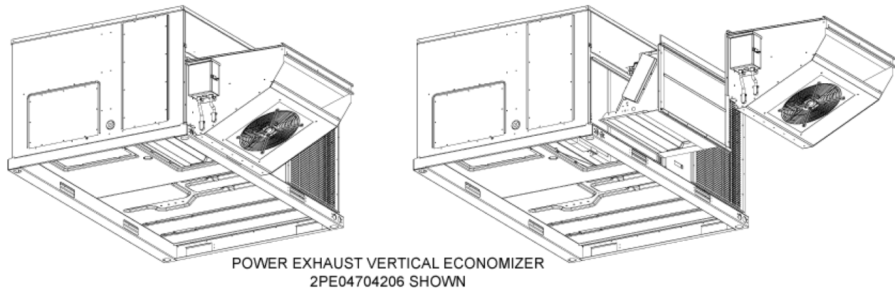
Figure 33: Field-installed horizontal flow economizer
