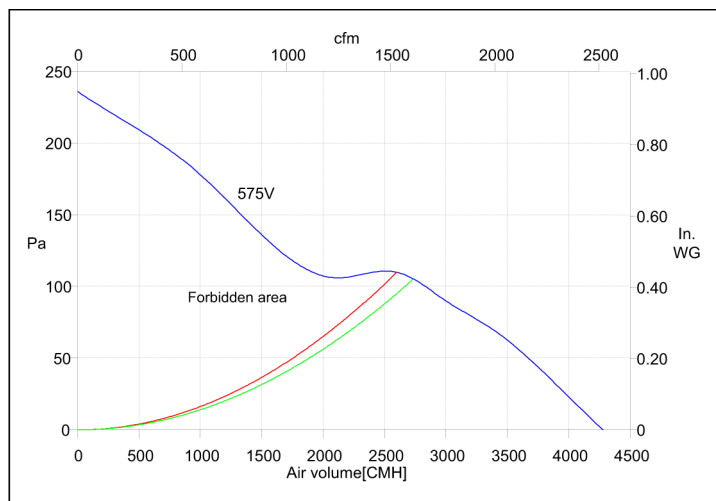
Figure 5: 575-3-50 power exhaust fan curve
