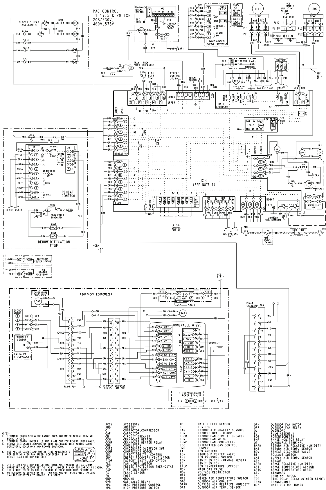
RAV210-240 Control Wiring Diagram, Electro-Mechanical with W7220 Controller
