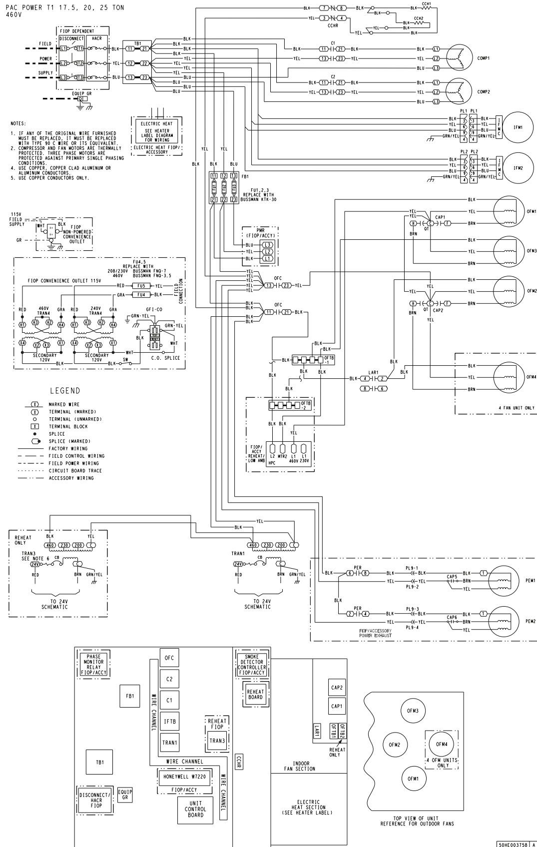
RAV210-300 Power Wiring Diagram, Electro-Mechanical with W7220 Controller
