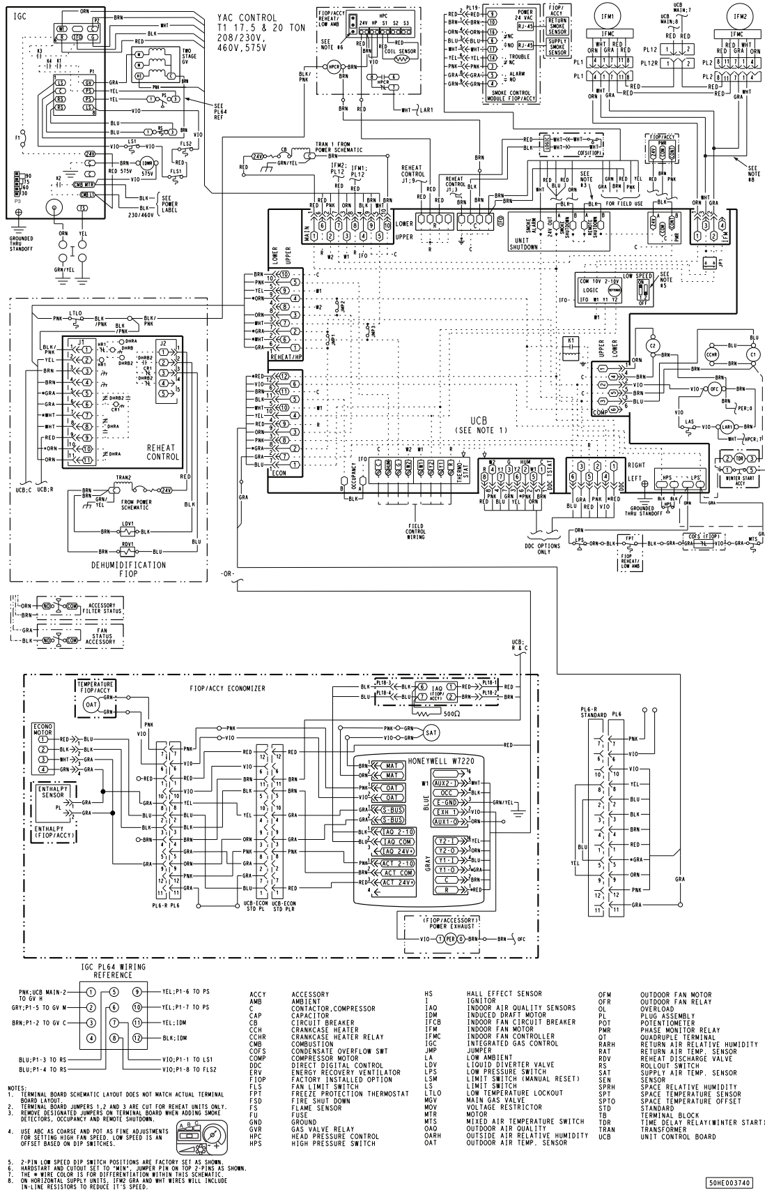
RGV210-240 Control Wiring Diagram, Electro-Mechanical with W7220 Controller
