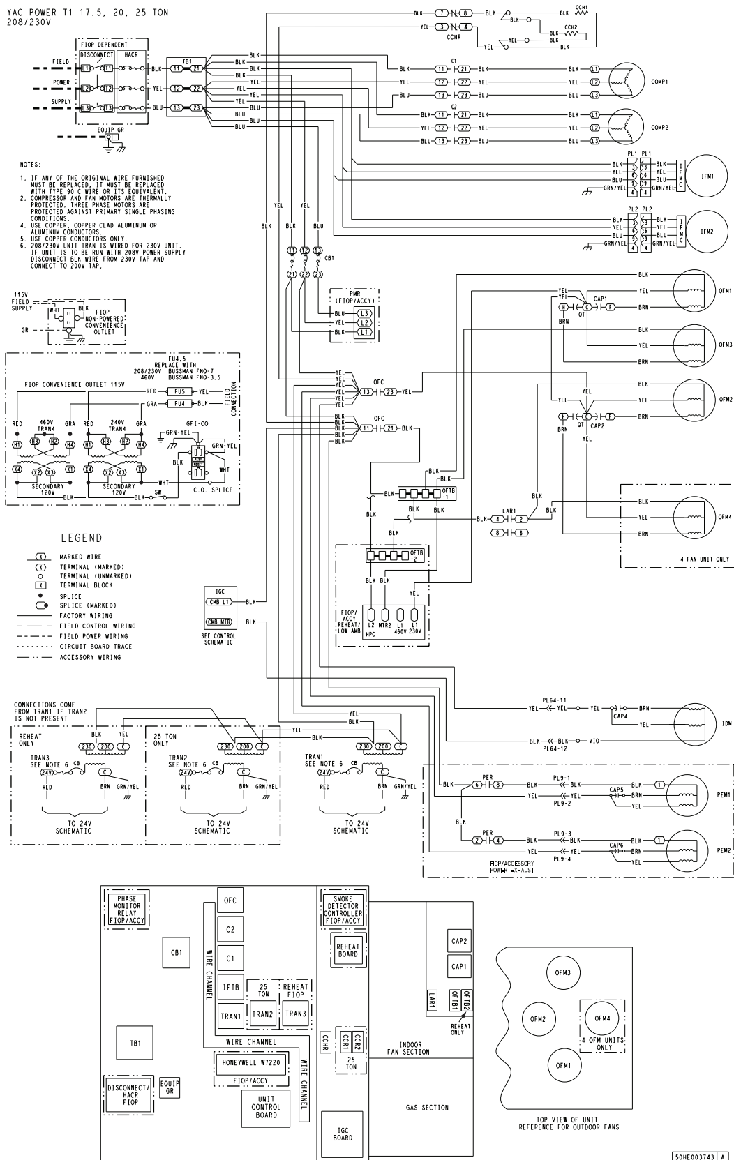
RGV210-300 Power Wiring Diagram, Electro-Mechanical with W7220 Controller
