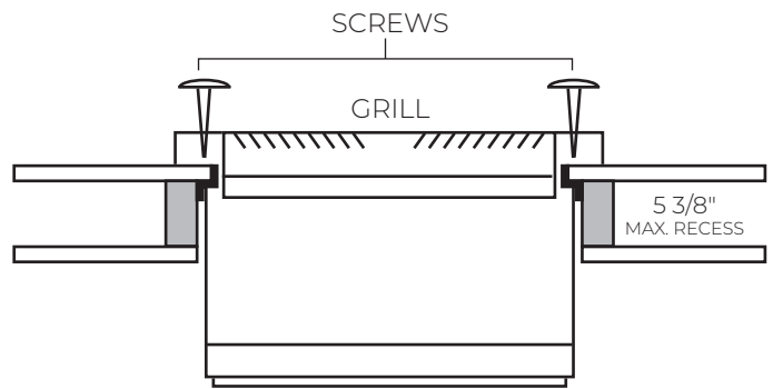
FIGURE 9 - RECESSED MOUNTING
