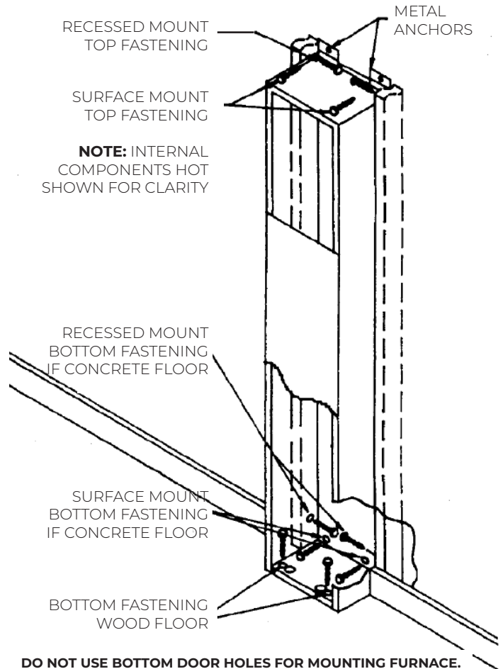
FIGURE 7 - HEATER MOUNTING
